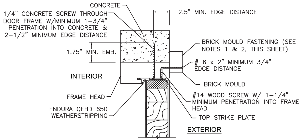
3 HEAD ANCHORAGE AT STRIKE PLATE
