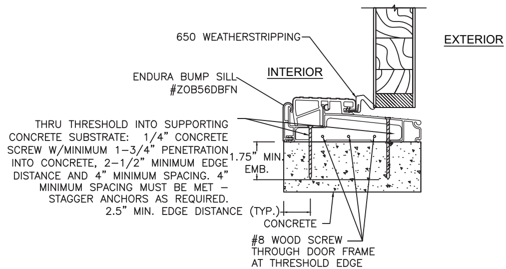
6 THRESHOLD SECTION AT SILL
