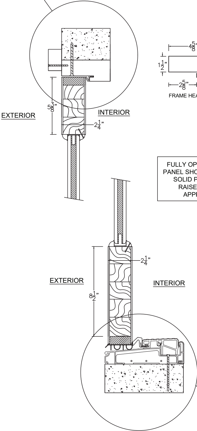
B INFILL DOOR SECTION CONCRETE/MASONRY SUBSTRATE INSTALLATION
