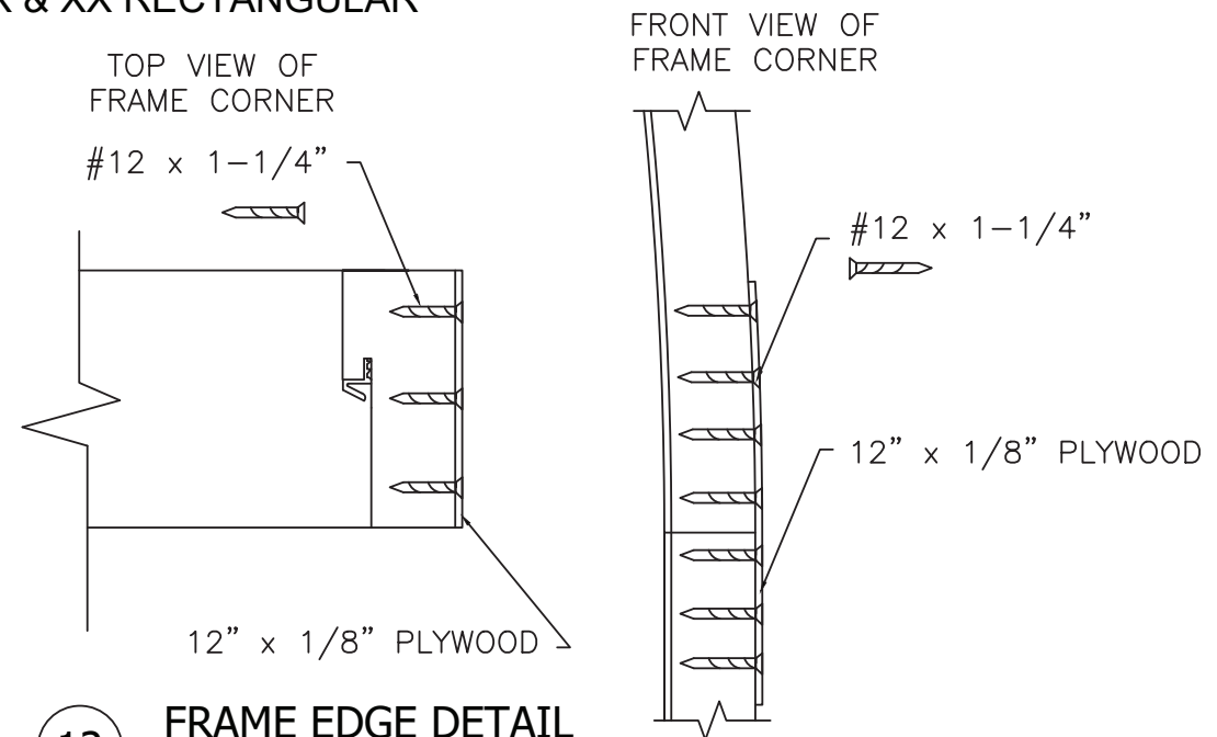
12 FRAME EDGE DETAIL X & XX RECTANGULAR
