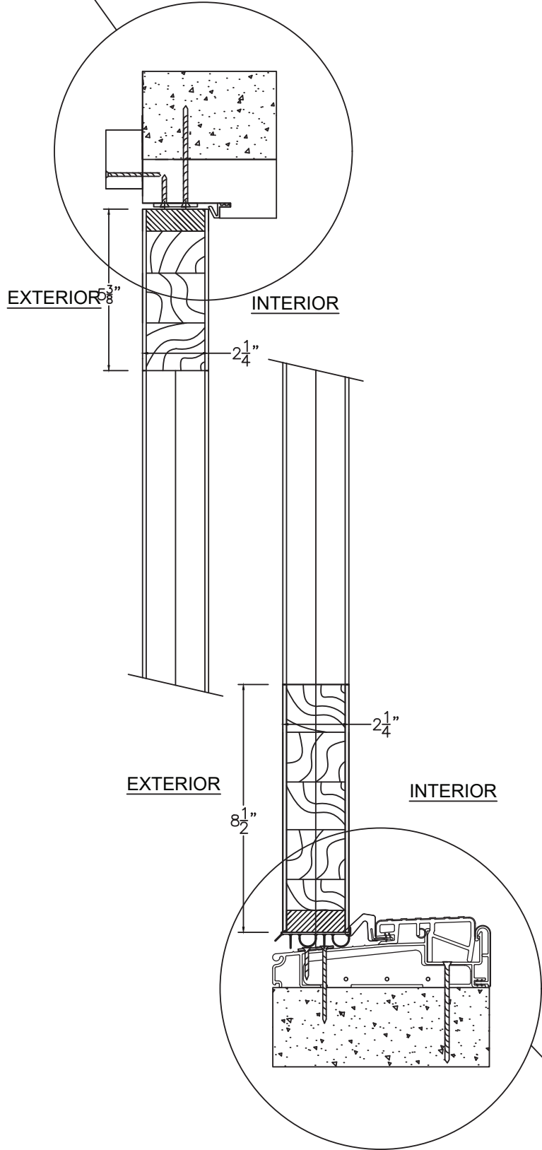
A STILE DOOR SECTION CONCRETE/MASONRY SUBSTRATE INSTALLATION
