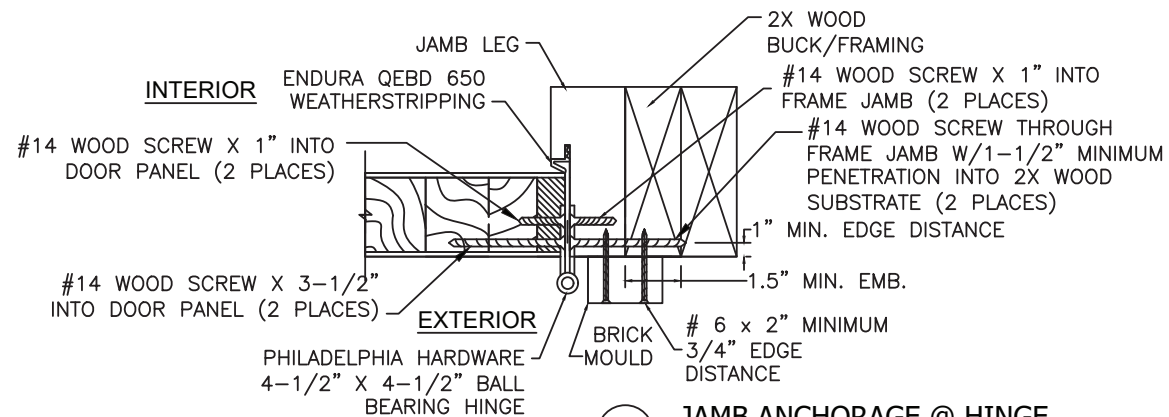
8 JAMB ANCHORAGE @ HINGE
