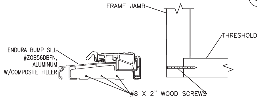
11 THRESHOLD TO FRAME DETAIL ZOB56DBFN (BRONZE 5-5/8" BUMPER OUTSWING SILL) OR ZOB76DBFN (BRONZE 7-5/8" BUMPER OUTSWING SILL) USED
