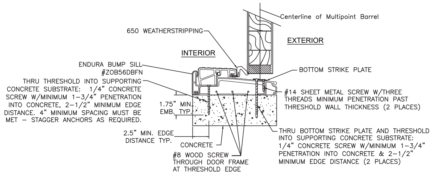
4 THRESHOLD SECTION AT STRIKE PLATE
