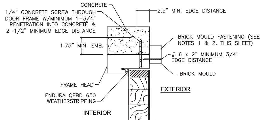
5 HEAD ANCHORAGE AT FRAME HEAD
